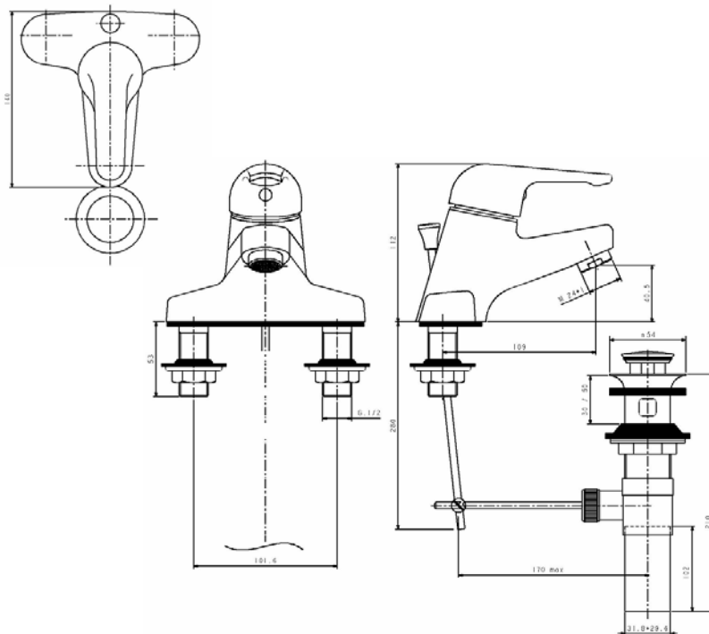
18046 Basin mixer 4" center set
