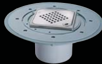
2 Variofix shallow bed upper section made of ABS, frame □ 132 mm, flange Ø 312 mm
