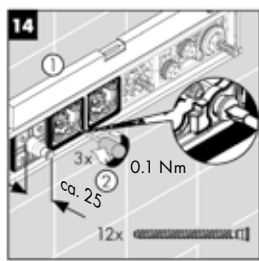
Tightening the screws of the Select valves to 0.1 Nm
