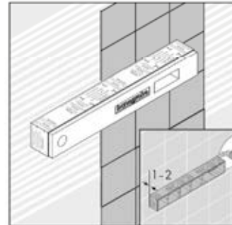
Trim the sealing collar to size. Slide over the housing, and press into the adhesive and silicone. Tile the wall. Shorten the housing to 1–2 mm.
