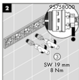
Fitting the Select valves
