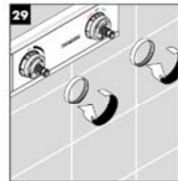
Screwing in the attachment rings for the glass cover
