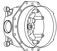
iBox® universal Basic set iBox universal # 01800180 Extension set 25 mm for too deep installation: # 13595000 Extension set 22 mm for too low installation depths: # 13597000 for Ecostat S, diameter 150 mm # 15497000 for Ecostat measuring 155 mm x 155 mm # 15597000 for Ecostat E and PuraVida measuring 155 mm x 155 mm # 13596000 for escutcheons of diameter 170 mm
