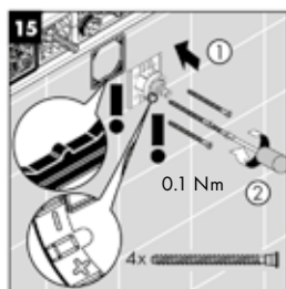
Tightening the screws of the flow valve to 0.1 Nm
