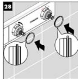
Fitting the glass cover and applying the seals
