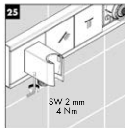
Attaching the shower holder at 4 Nm
