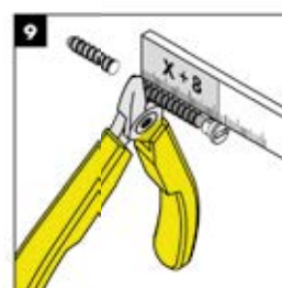
Shortening the fixation screws
