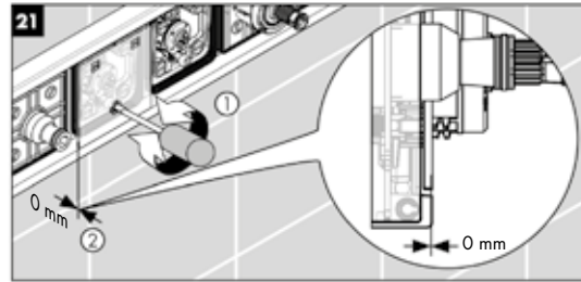
Adjusting the template for the glass button
