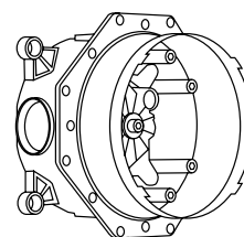
iBox® universal Basic set iBox universal # 01800180 Extension set 25 mm for too deep installation: # 13595000 Extension set 22 mm for too low installation depths: # 13593000 for ShowerSelect in the dimensions 155 mm x 155 mm # 13597000 for ShowerSelect of diameter 150 mm # 13601000 for ShowerSelect including FixFit and holder # 13604000 for ShowerSelect glass
