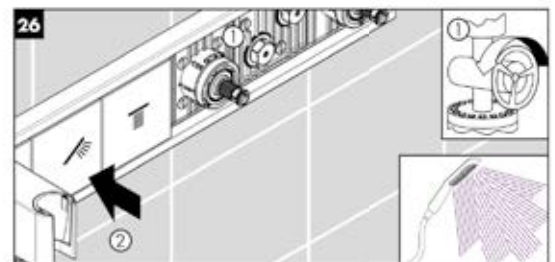
Starting the water flow and activating the button for the hand shower
