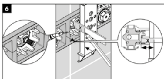
Measuring the optimum screw length for components that can be cut to length
