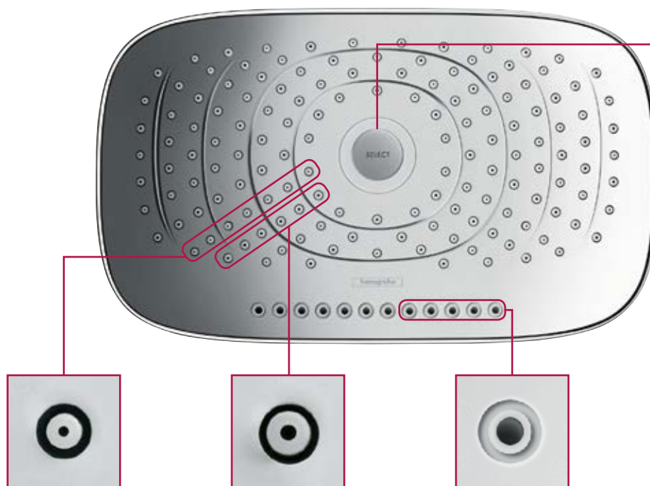
Small opening for Rain spray
