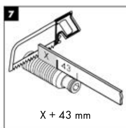
Shortening the shower holder connection
