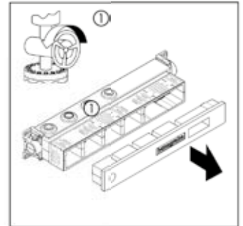
Remove the plaster cap.
