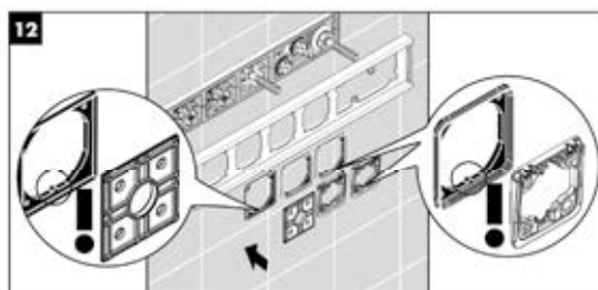
Pre-assembling the covers
