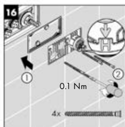
Tightening the screws of the thermostat valve to 0.1 Nm
