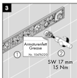
Fitting the quality valve
