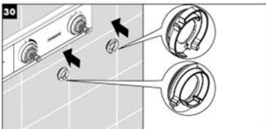
Using the temperature and flow limiter
