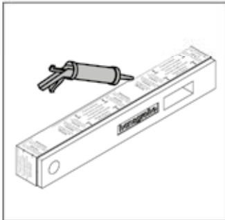
Plastering over fitted, tested basic set (finish wall installations with cladding). Fill the dried seam between the wall and housing with silicone (without acetic acid).
